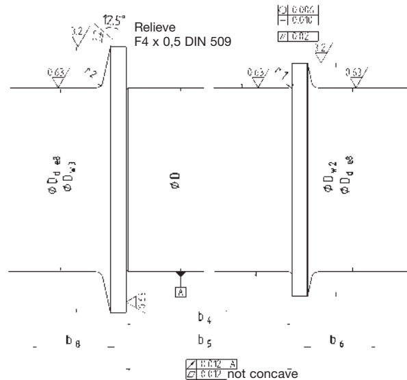
Locating bearing Type of bearing shell E...B E...K E...E
