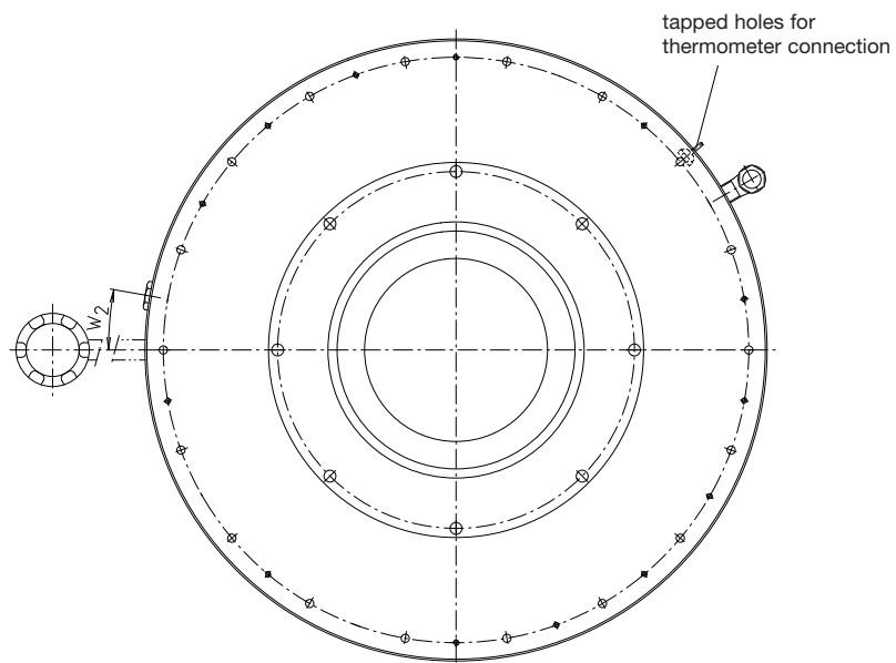
drawing shows type VGWCU 18-16
