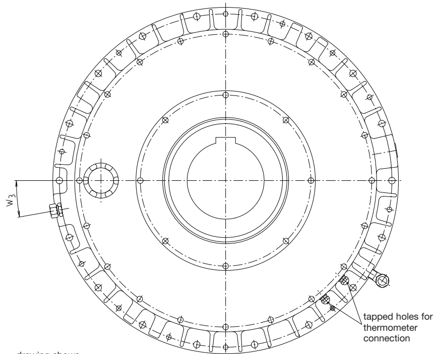
drawing shows type VTWCU 18-28
